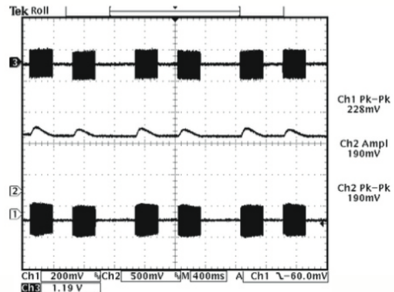
AGC attacking and decaying with gating enabled.
