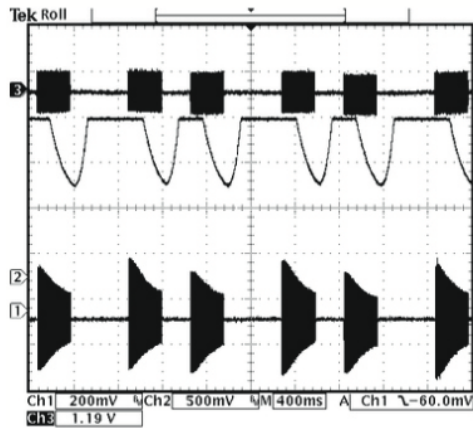
AGC attacking and decaying with gating disabled.
