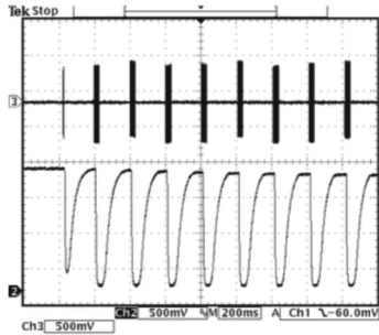
Peak time constants dominating control due to very high setting of average attack.
